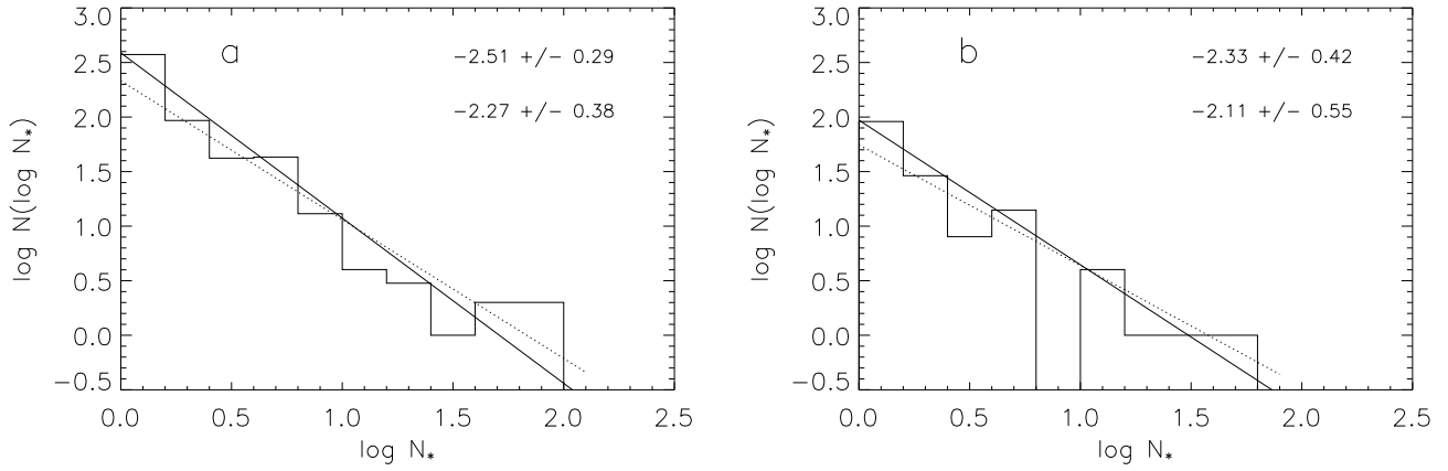
FIG. 5.— The distribution in N_* for groups defined from the candidate OB sample (panel a ) and O-star sample (panel b ). Fits to the power-law exponent ( -\beta ) are shown for the entire distributions (upper values) and omitting the first bin of single stars (lower values). Note that the slope fitted in logarithmic space is -\beta + 1 .
