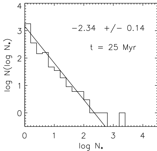
FIG. 8.— Monte Carlo models for evolution in the \log N_* distribution, assuming that all objects were created simultaneously. Models for ages of 0, 15, and 25 Myr are shown, with fitted power-law slopes. As in Figure 5, the linear power-law exponents are shown, while the fitted slope is -\beta + 1 in logarithmic space.
