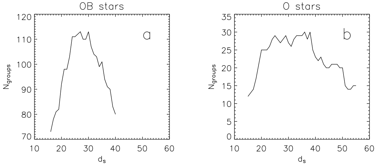
FIG. 2.— Number of groups with N_* \geq 3 as a function of clustering distance d_s for the OB sample (panel a) and O-star sample (panel b).
